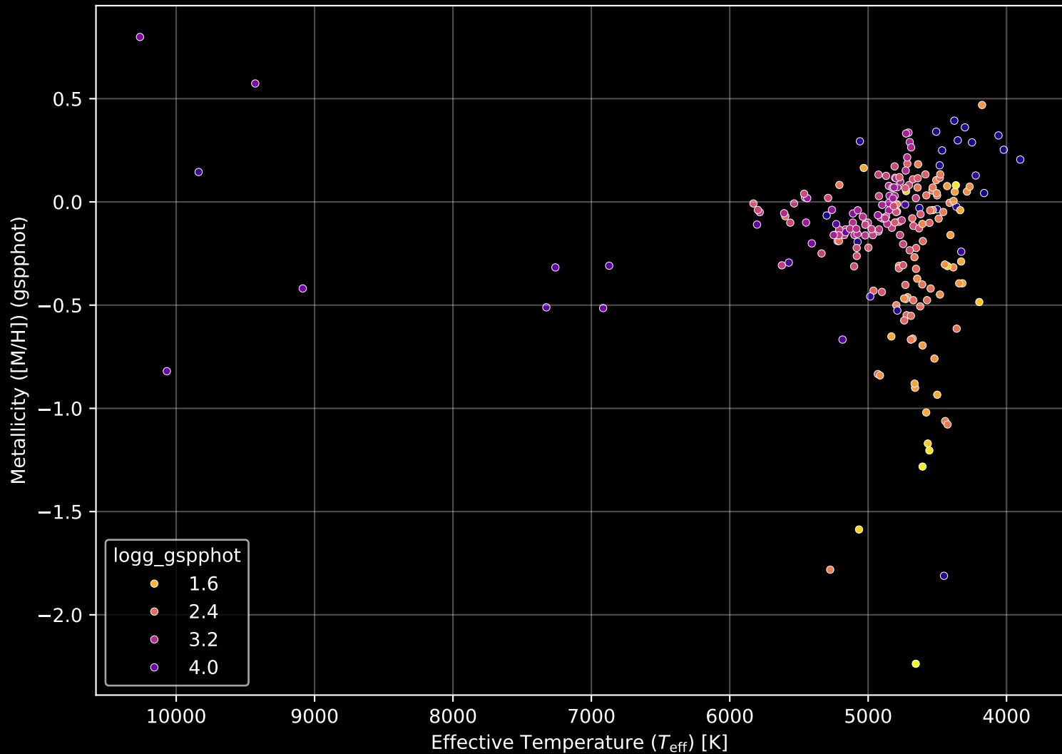
APOGEE DR17 Field: [300+12] Stellar Population Parameters (n= 213)
