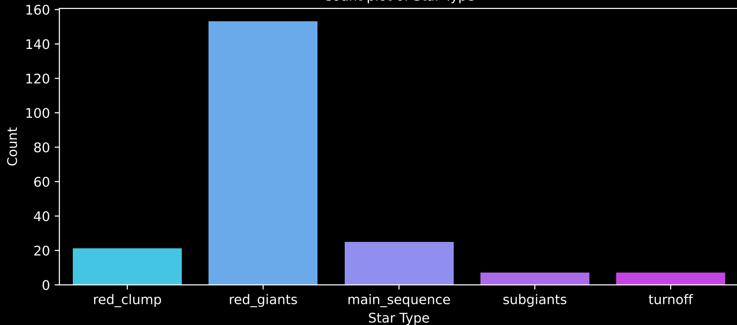
APOGEE DR17 Field: [300+12] Count plot of Star Type
