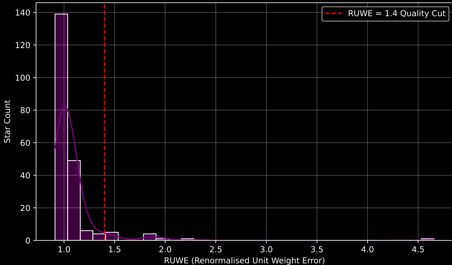
GAPOGEE DR17 Field [300+12] RUWE Distribution (n= 210)
