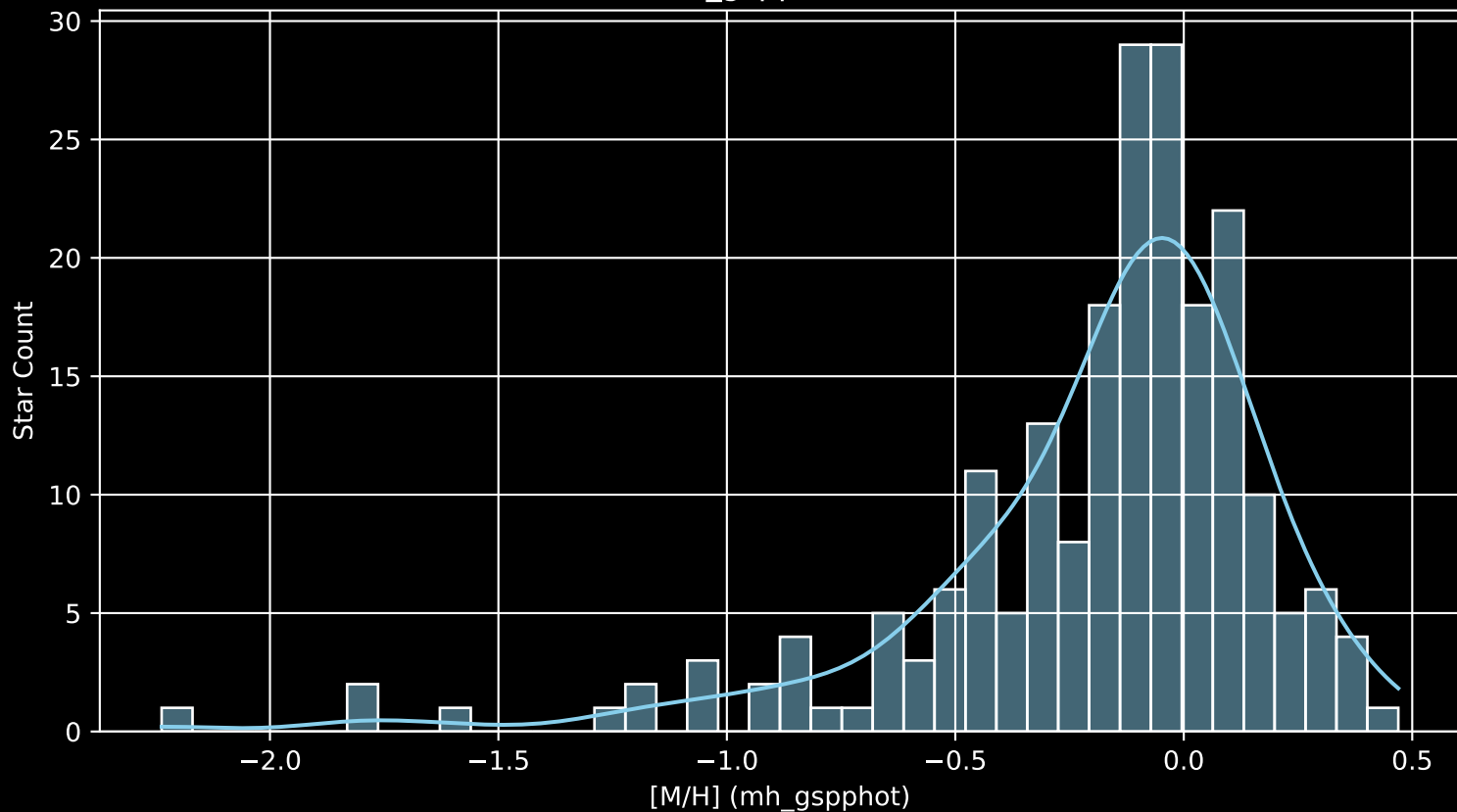
APOGEE DR17 Field: [300+12 [M/H] (mh_gspphot) (n= 211)
