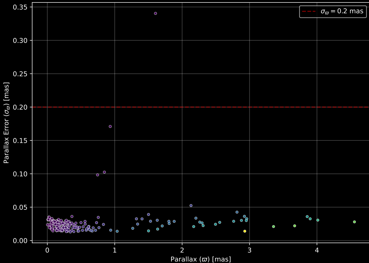
APOGEE DR17 Field: [300+12] Parallax Quality (n= 213)
