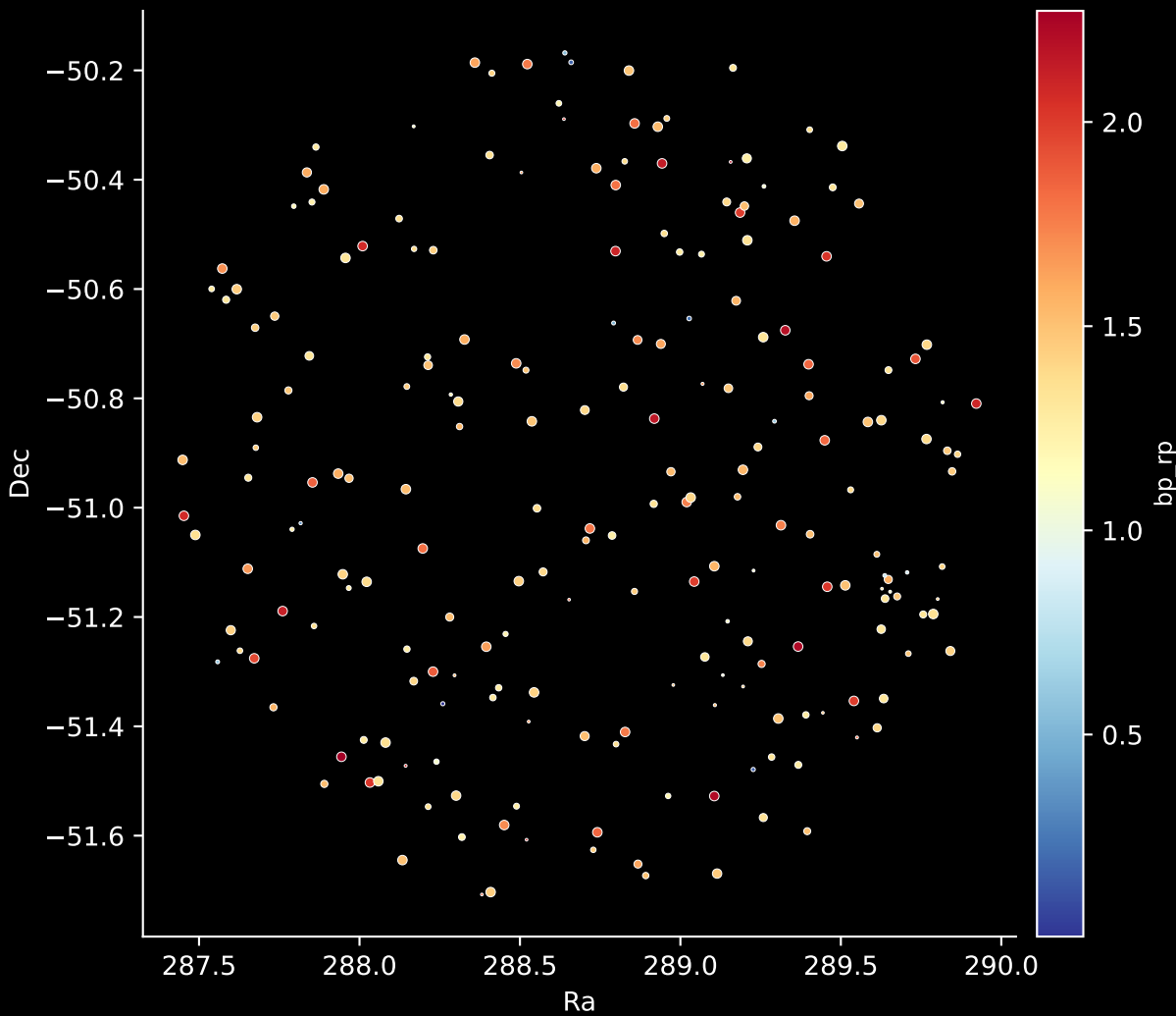
APOGEE DR17 Field: [300+12] Stars: 213
