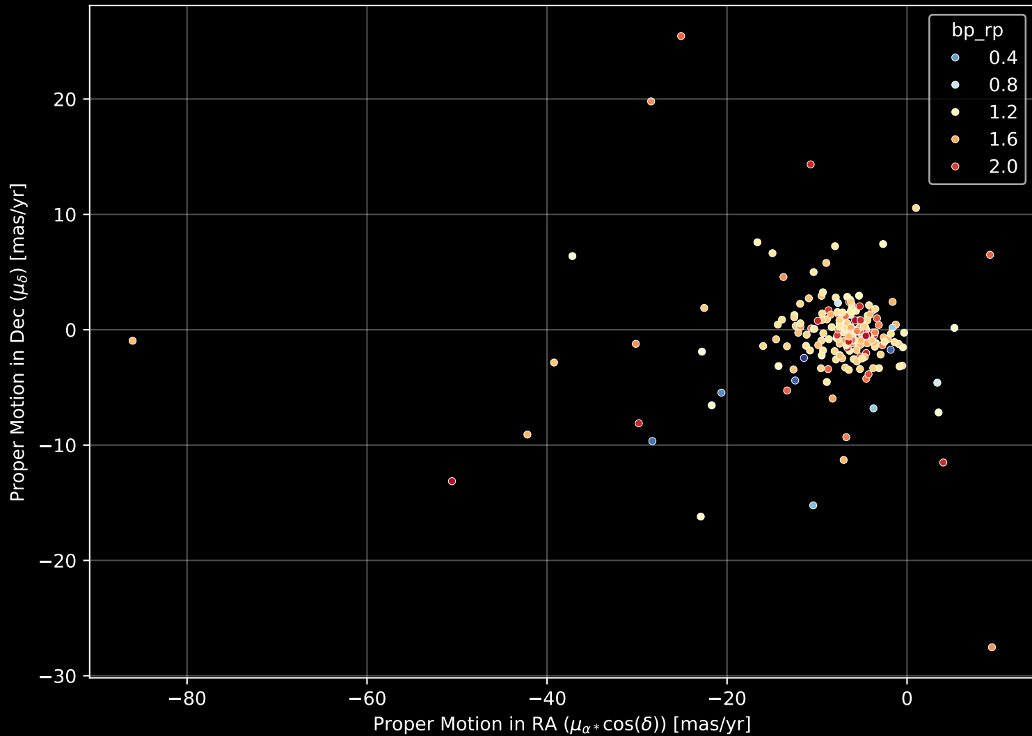
APOGEE DR17 Field: [300+12] Proper Motion Diagram (n= 213)
